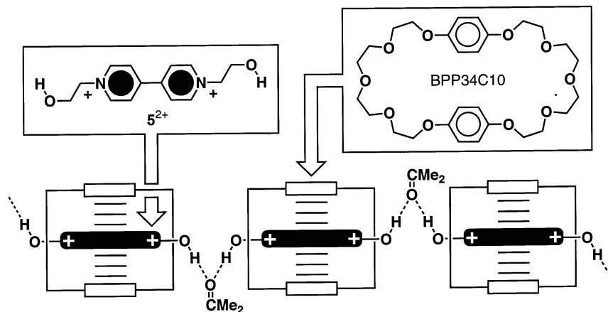
Fig. 4. Cartoon illustrating the interwoven supramolecular array that is formed when the pseudorotaxane [BPP34C10 \cdot 5]^{2+} associates with Me_2CO in the solid state via hydrogen bonds. Interchain associations are not shown in the cartoon for the sake of clarity.
