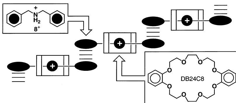
Fig. 7. Cartoon portraying the X-ray crystal structure of the pseudopolyrotaxane \{[\text{DB24C8} \cdot \mathbf{8}]^+\}_n .
