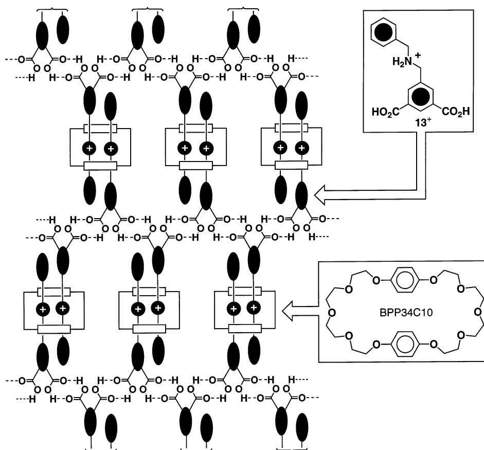
Fig. 13. Cartoon representation of the interwoven supramolecular cross-linked polymer \{[\text{BPP34C10} \cdot (13)_2]^+\}_n .
